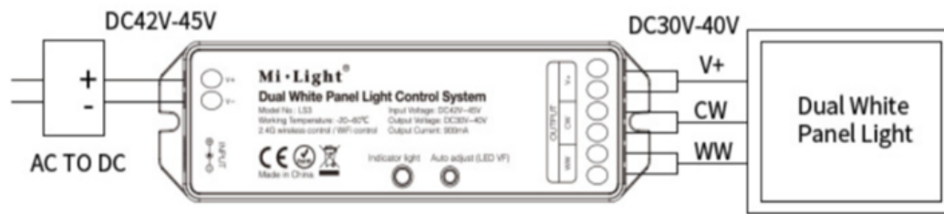
Dual White Panel Light wiring diagram
